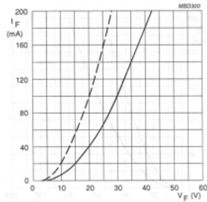
BY8004. Dotted line: T_J = 120 °C. Solid line: T_J = 25 °C.
