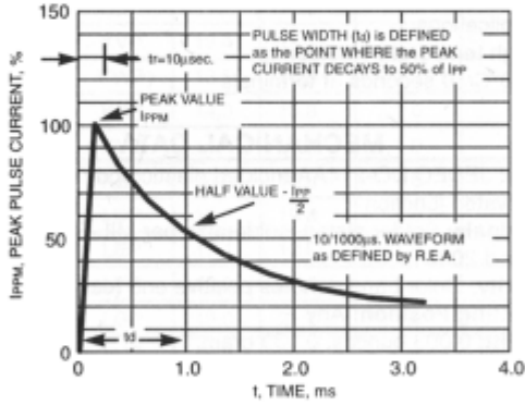
FIG. 3 - PULSE WAVEFORM
