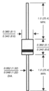
Case Style P600
